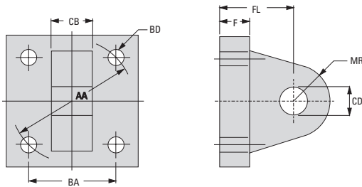
Eye Bracket
