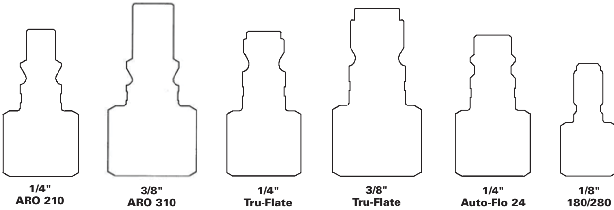
Industrial Interchange
